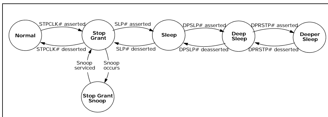
Figure 2. Package Low Power States
